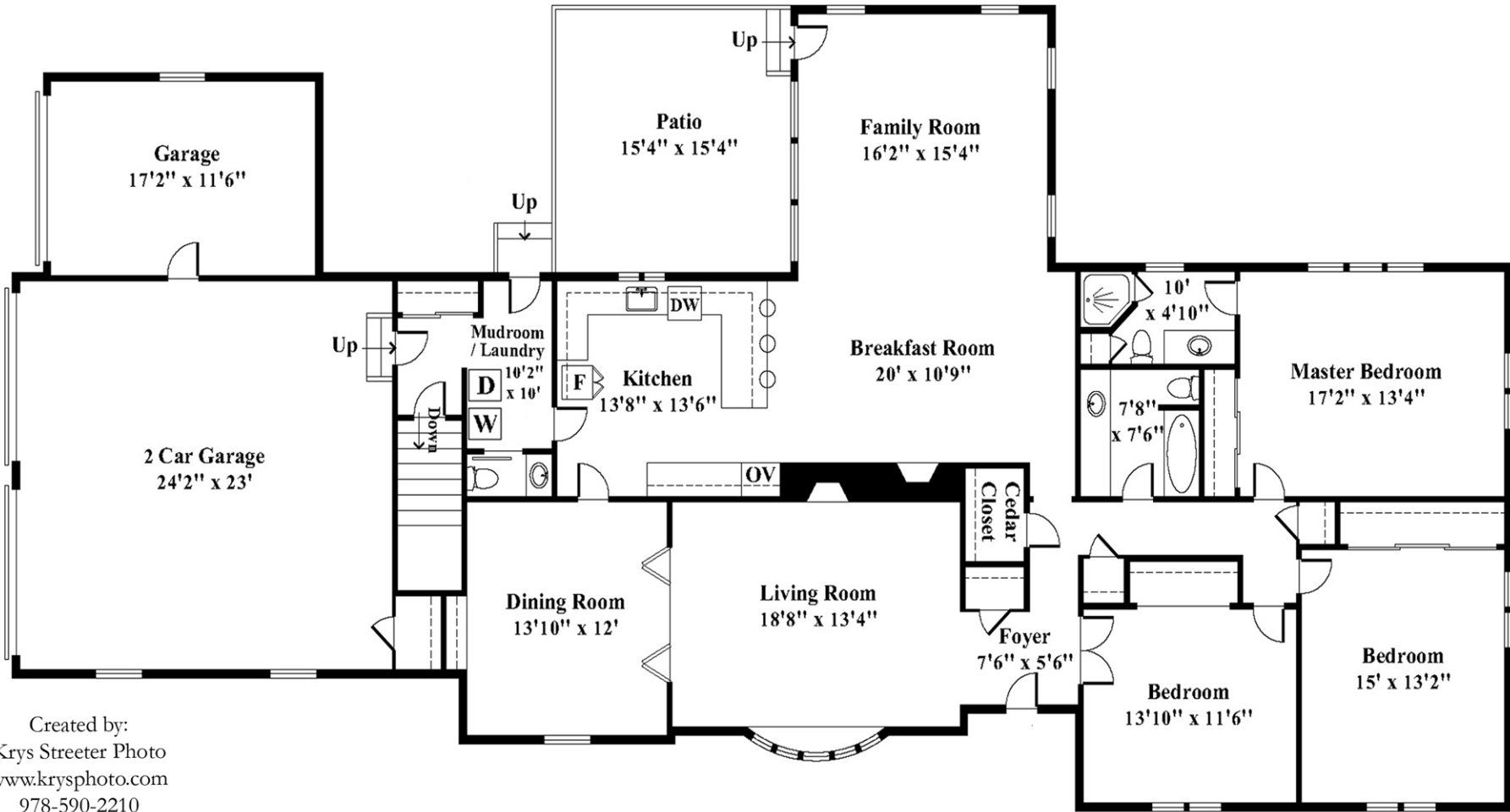
First Level
