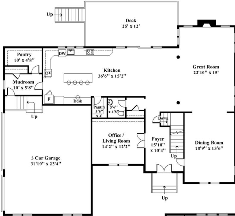
First Level
