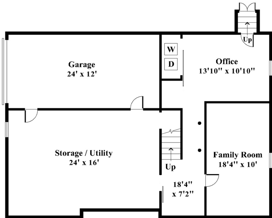
Lower Level
