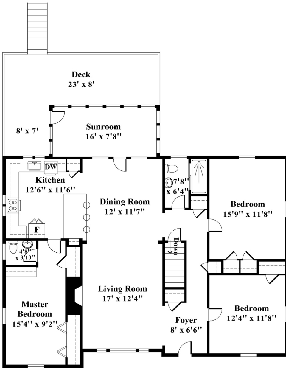
First Level
