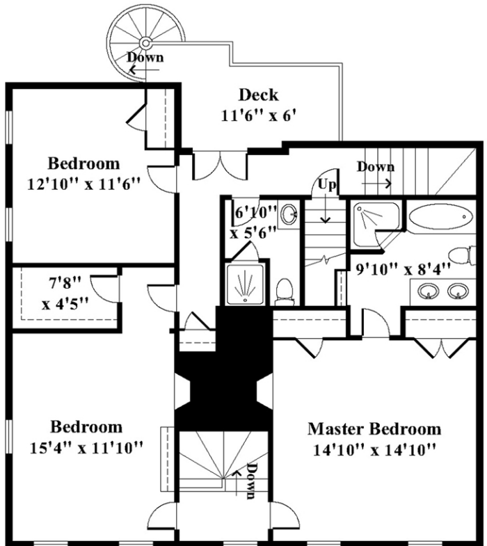
Second Level
